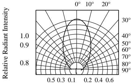
FIG.6 RADIATION DIAGRAM
