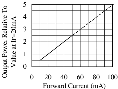
FIG.4 RELATIVE RADIANT INTENSITY VS. FORWARD CURRENT
